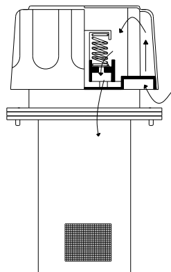
OPTION 'P' Pressurization valve (0.35 bar)
